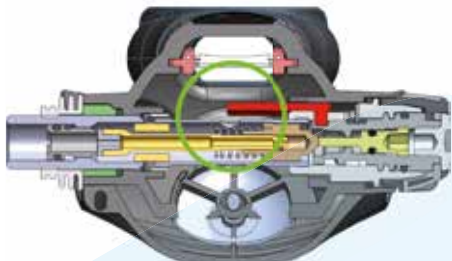
MBS en position minimale / MBS on minimum position
